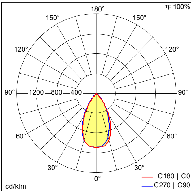
TE_LILY_LED_SPOT_IP44_60_68_850_930.idt
